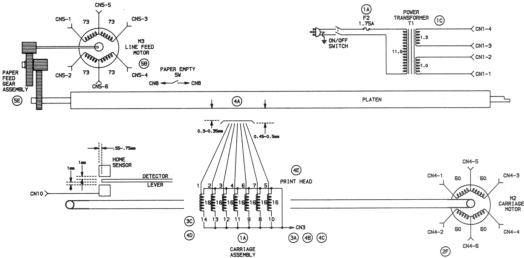
INTERCONNECTING DIAGRAM
